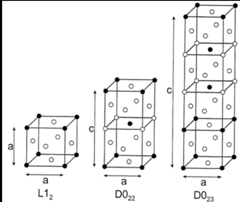
Fig. 1. Crystal structures for ZrAl_3 compounds: cubic L1_2 , tetragonal D0_{22} at ideal c/a=2 , tetragonal D0_{23} at ideal c/a=4 . (○) Al atoms; (●) Zr atoms.
